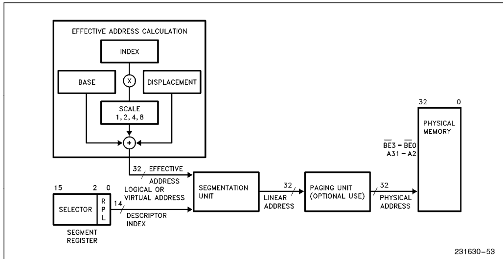
Figure 2-11. Address Translation
