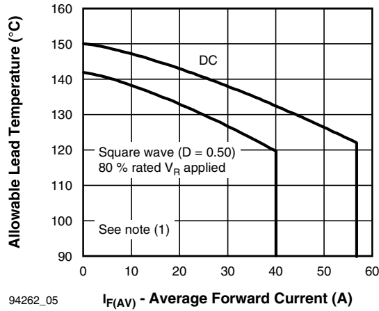
94262_05 I F(AV) - Average Forward Current (A) Fig. 5 - Maximum Allowable Lead Temperature vs. Average Forward Current
