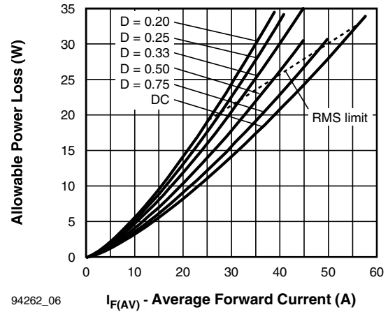
94262_06 I F(AV) - Average Forward Current (A) Fig. 6 - Maximum Average Forward Dissipation vs. Average Forward Current
