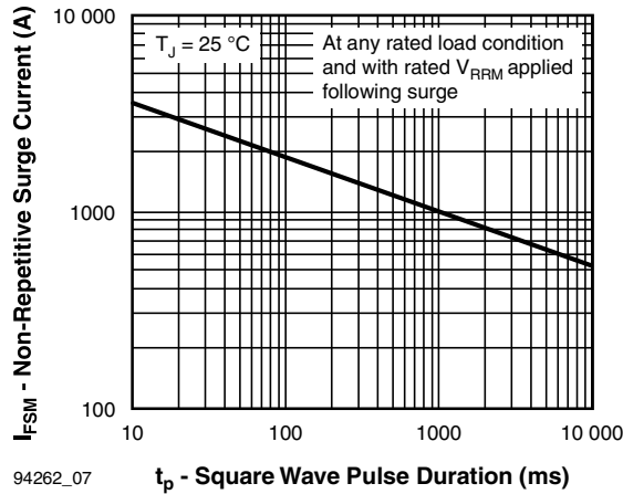
94262_07 t p - Square Wave Pulse Duration (ms) Fig. 7 - Maximum Peak Surge Forward Current vs. Pulse Duration
