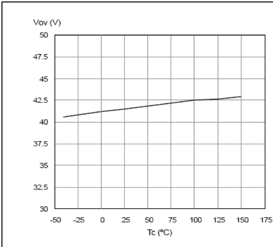
Figure 14. Turn-on voltage slope
