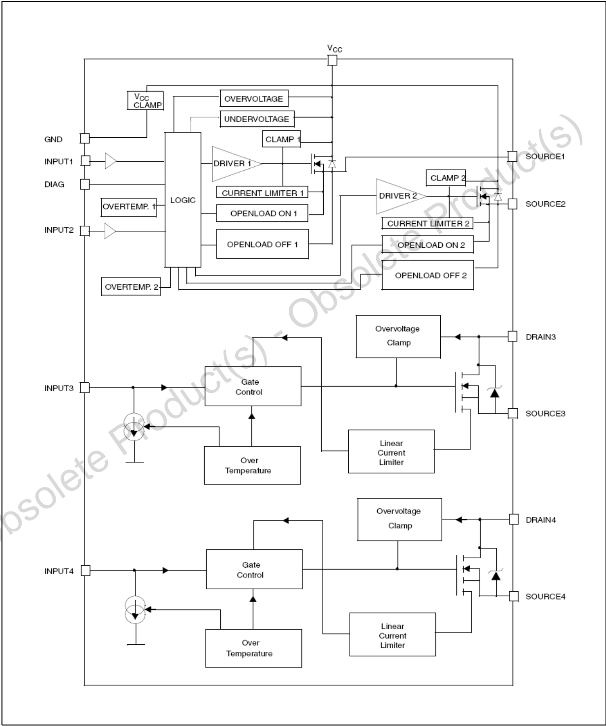
Figure 1. Block diagram
