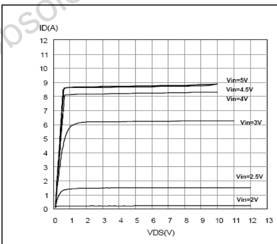
Figure 33. Output characteristics
