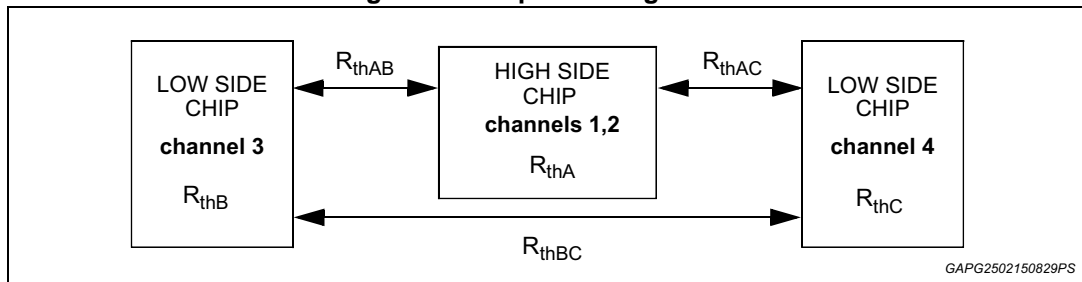
Figure 38. Chipset configuration
