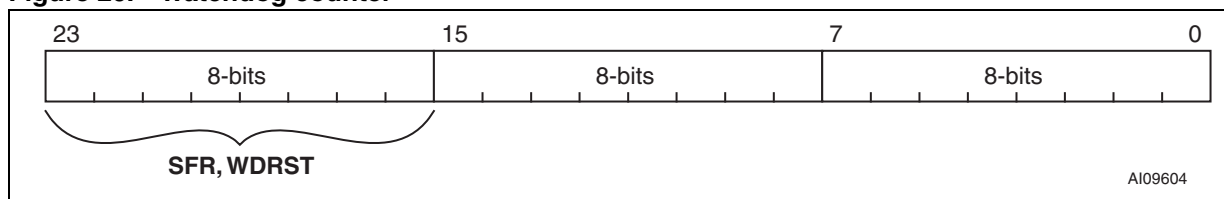
Figure 20. Watchdog counter
