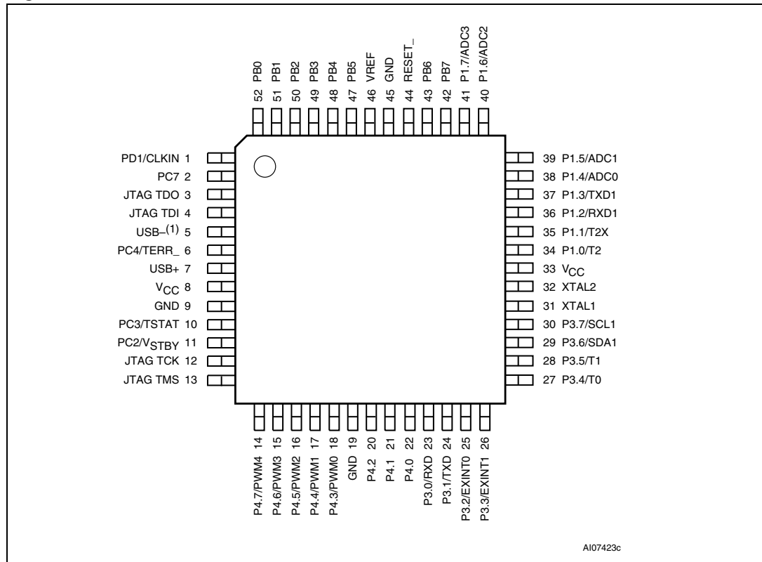
Figure 2. TQFP52 connections
