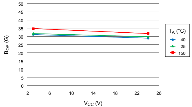
Average Operate Point versus Average Supply Voltage
