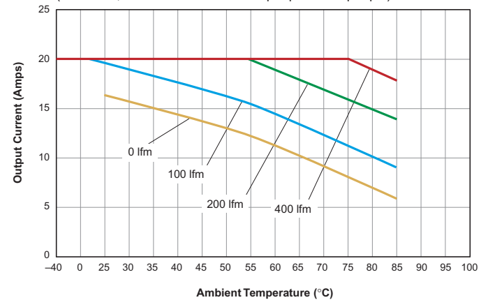
ULQ-3.3/20-D48
