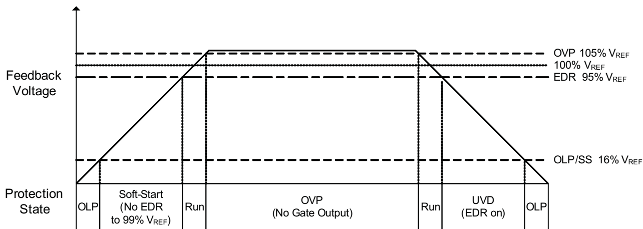
Figure 22. Soft Start and Protection States
