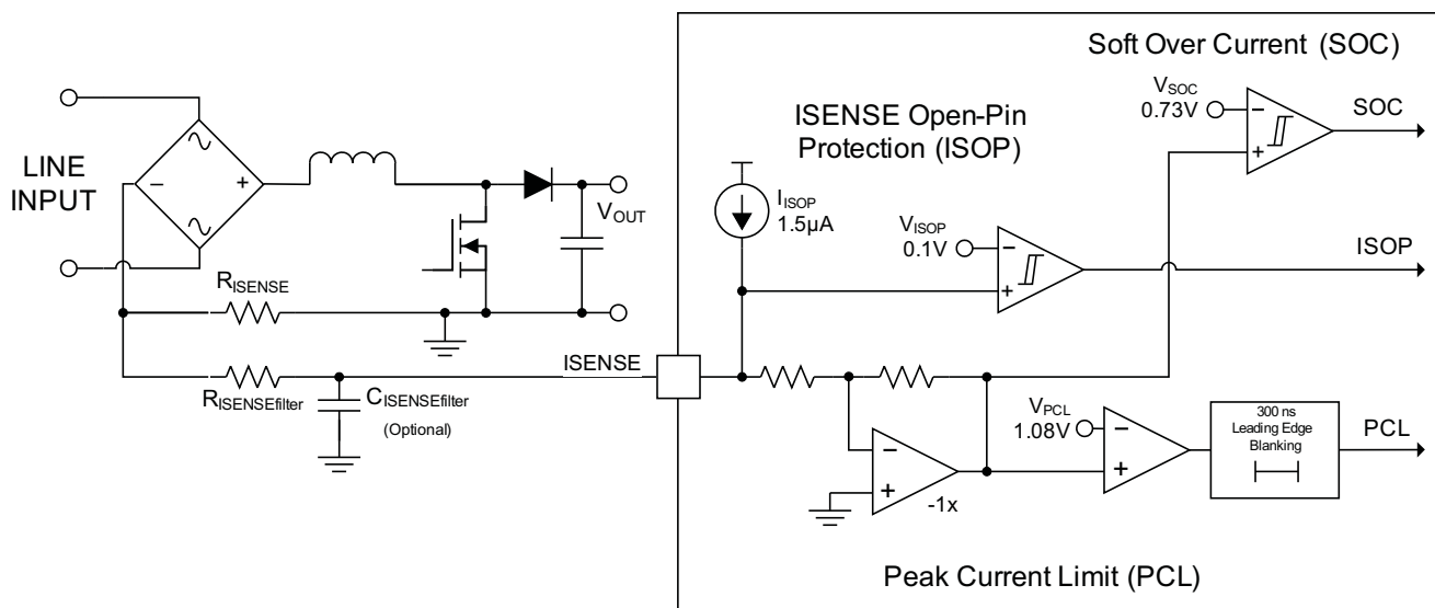
Figure 23. Soft Over Current/ Peak Current Limit
