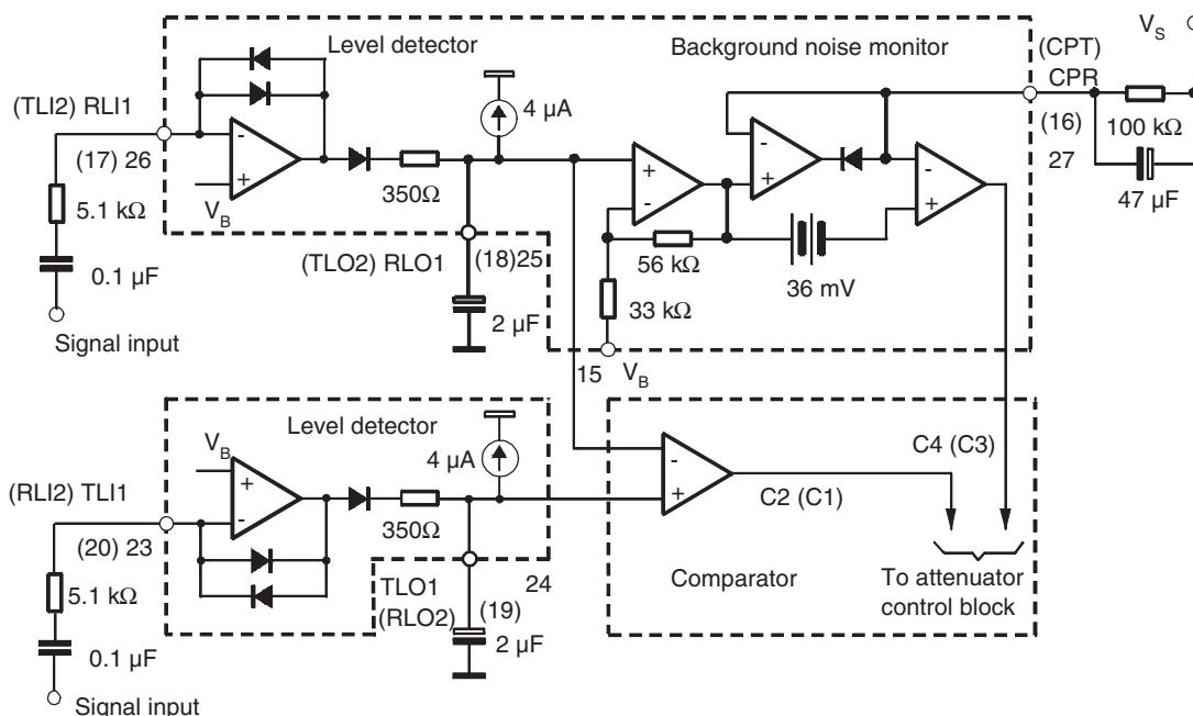
Figure 3-2. Level Detectors
