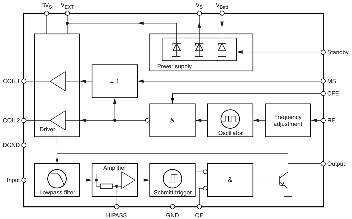
Figure 1-2. Block Diagram
