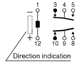
1 coil latching
