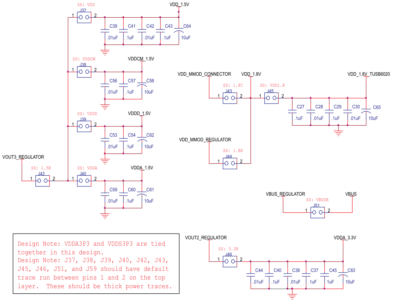
Figure 1-7. Power Jumpers
