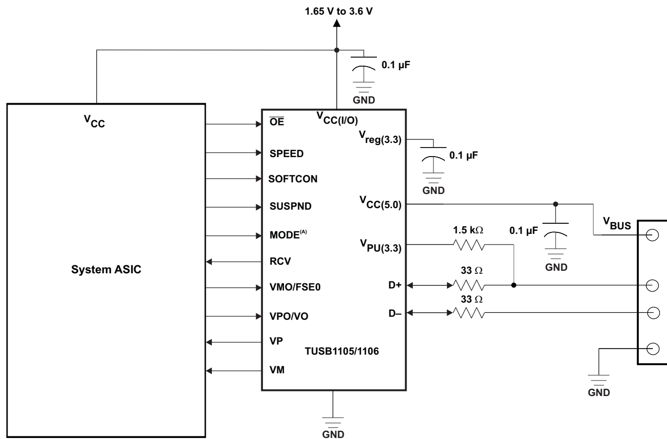
Figure 10. Peripheral-Side (Full-Speed) Internal Regulator Mode
