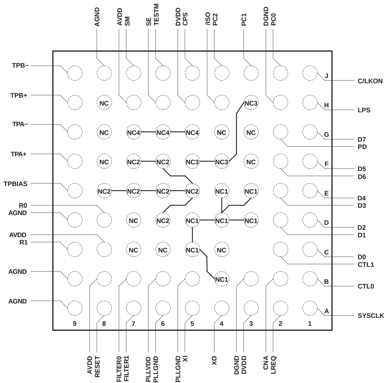
GQE PACKAGE TERMINAL DIAGRAM
