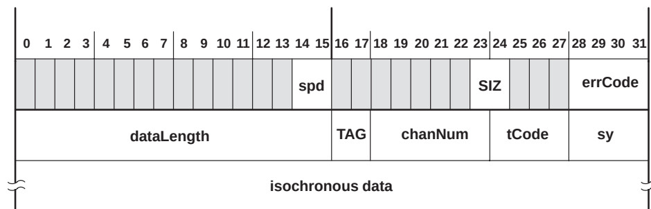
Figure 3–37. Isochronous-Receive Format for Bulky Data FIFO
