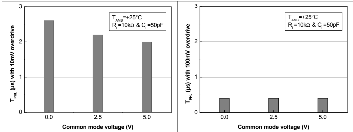
Figure 13. T_{PHL} vs V_{icm} at V_{CC} = 5\text{ V} and 10\text{ mV} overdrive Figure 14. T_{PHL} vs V_{icm} at V_{CC} = 5\text{ V} and 100\text{ mV} overdrive
