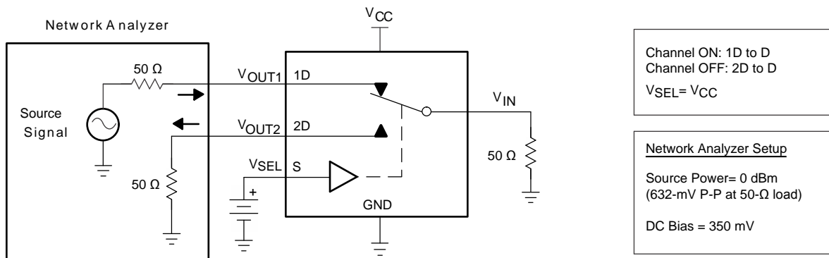
Figure 6. Crosstalk (XTALK)
