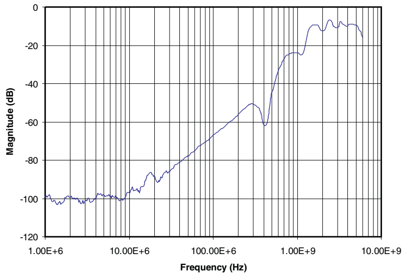
Figure 3. Crosstalk
