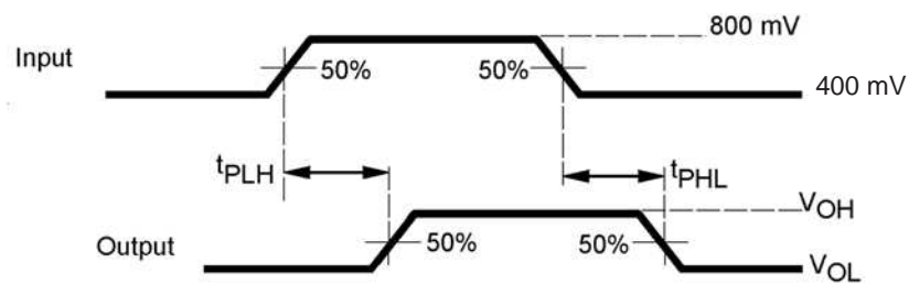
Figure 8. Propagation Delay
