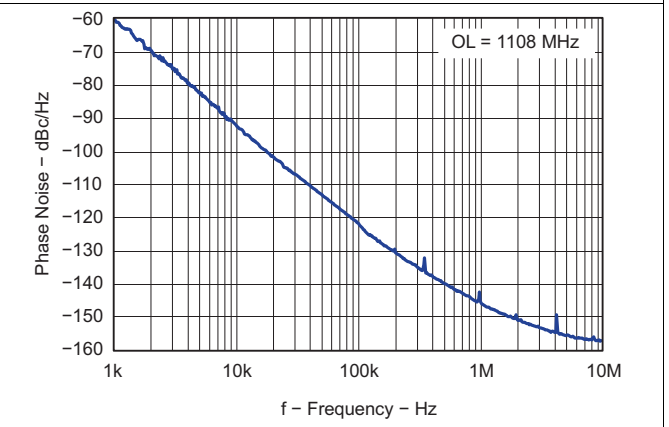
Figure 77. Open Loop VCO Phase Noise
