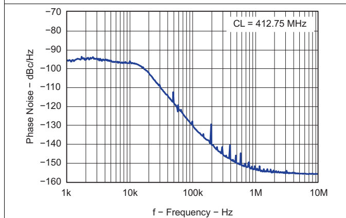
Figure 15. Closed Loop VCO Phase Noise
