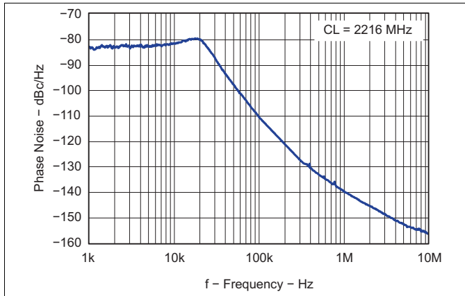
Figure 74. Closed Loop VCO Phase Noise
