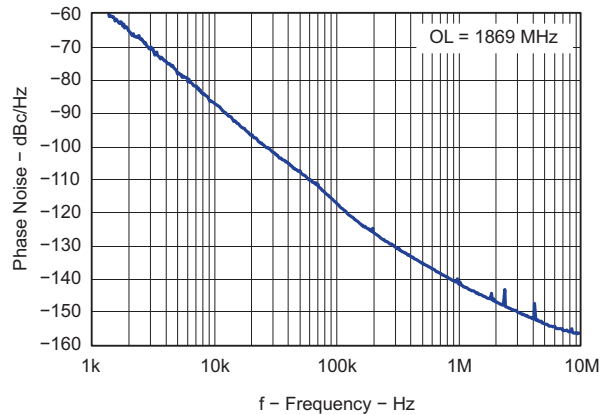
Figure 39. Open Loop VCO Phase Noise
