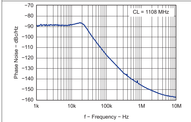
Figure 76. Closed Loop VCO Phase Noise
