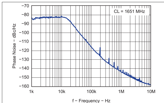
Figure 11. Closed Loop VCO Phase Noise
