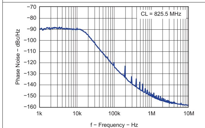
Figure 13. Closed Loop VCO Phase Noise
