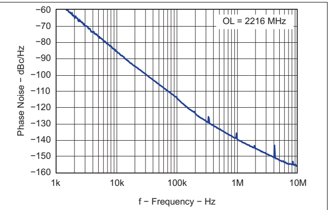
Figure 75. Open Loop VCO Phase Noise
