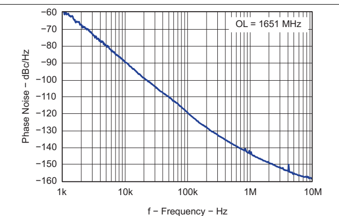
Figure 12. Open Loop VCO Phase Noise
