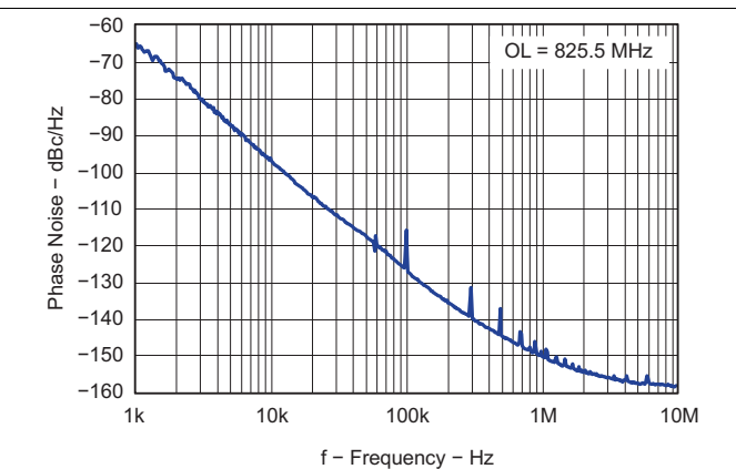
Figure 14. Open Loop VCO Phase Noise
