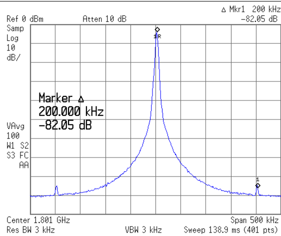
Figure 35. Direct Output: PFD Frequency Spurs
