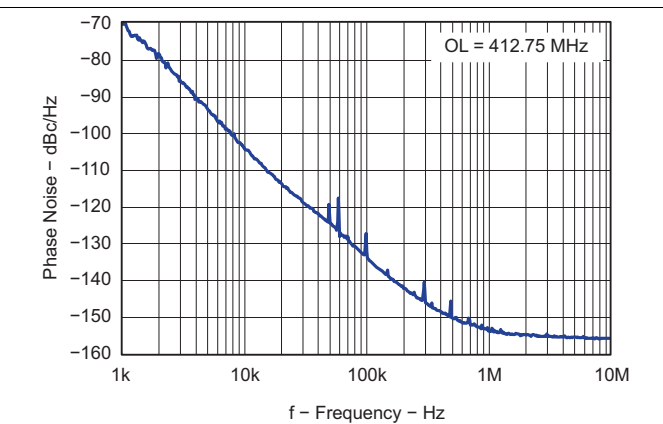
Figure 16. Open Loop VCO Phase Noise
