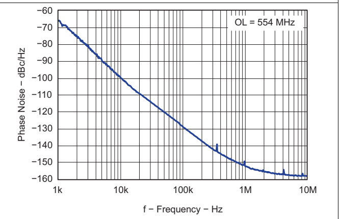
Figure 79. Open Loop VCO Phase Noise
