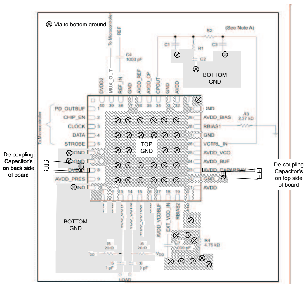
Figure 91. TRF3761 Layout
