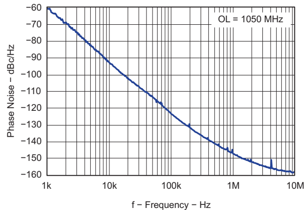
Figure 68. Open Loop VCO Phase Noise
