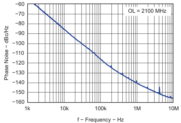
Figure 66. Open Loop VCO Phase Noise
