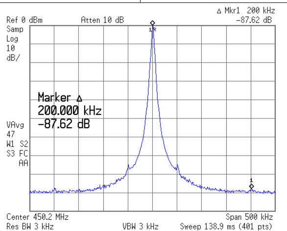
Figure 37. Divide-By-4 Output: PFD Frequency Spurs
