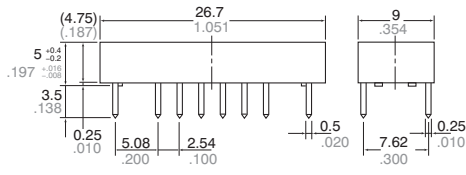
Self-clinching terminal
