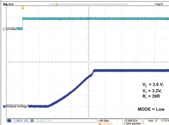
Figure 25. TPS82699 Start-Up
