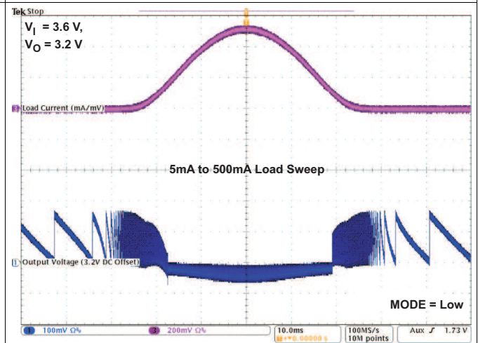
Figure 35. TPS82699 AC Load Transient Response
