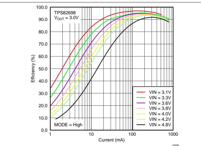
Figure 12. Efficiency vs Load Current Forced PWM Operation For Device TPS82698
