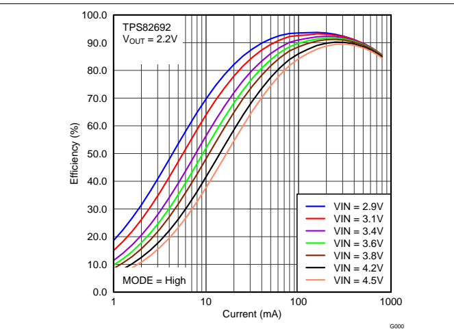
Figure 14. Efficiency vs Load Current PWM Operation For Device TPS82692
