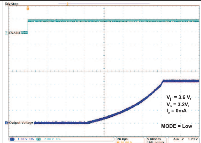
Figure 24. TPS82699 Start-Up
