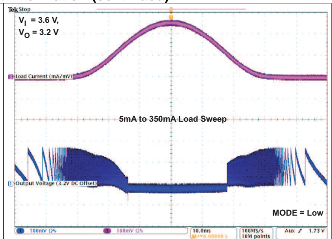
Figure 33. TPS82699 AC Load Transient Response
