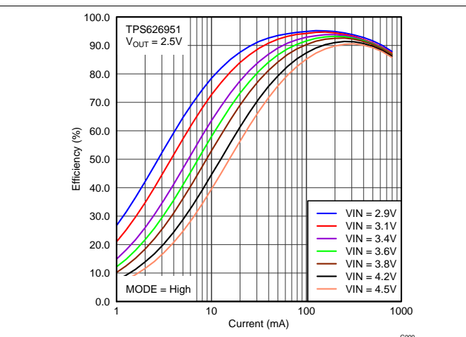
Figure 10. Efficiency vs Load Current Forced PWM Operation For Device TPS826951
