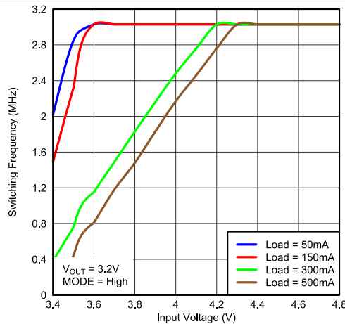
Figure 23. TPS82699 PWM Switching Frequency vs Input Voltage
