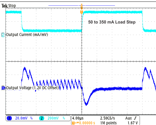
Figure 31. Load Transient Response in PFM/PWM Operation
