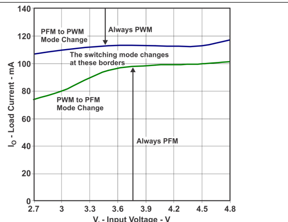
Figure 40. PFM/PWM Boundaries
