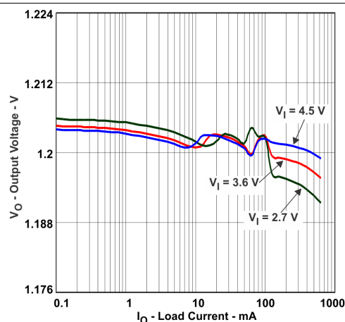
V_O = 1.2 V PFM/PWM Operation (TPS82677)
