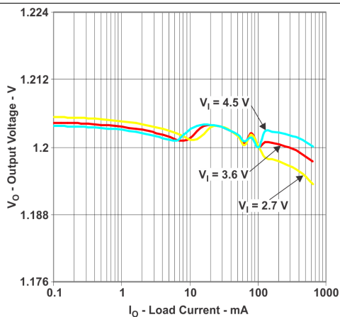
V_O = 1.2 V (TPS82675)
