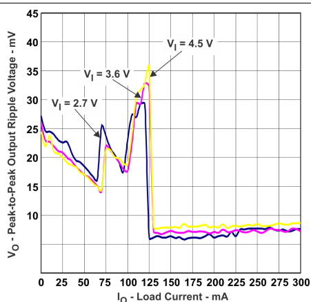
V_O = 1.2 V (TPS82671)
