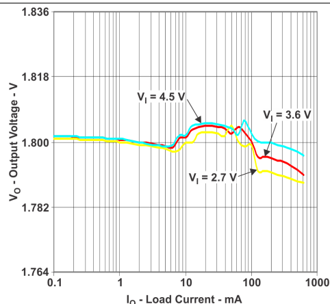
V_O = 1.8 V PFM/PWM Operation (TPS82671)
