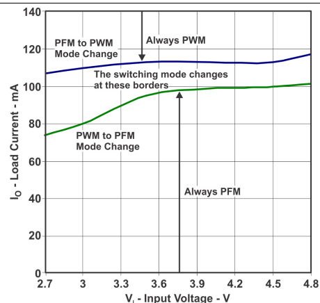
Figure 40. PFM/PWM Boundaries
