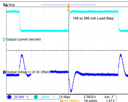
Figure 36. Load Transient Response in PFM/PWM Operation
