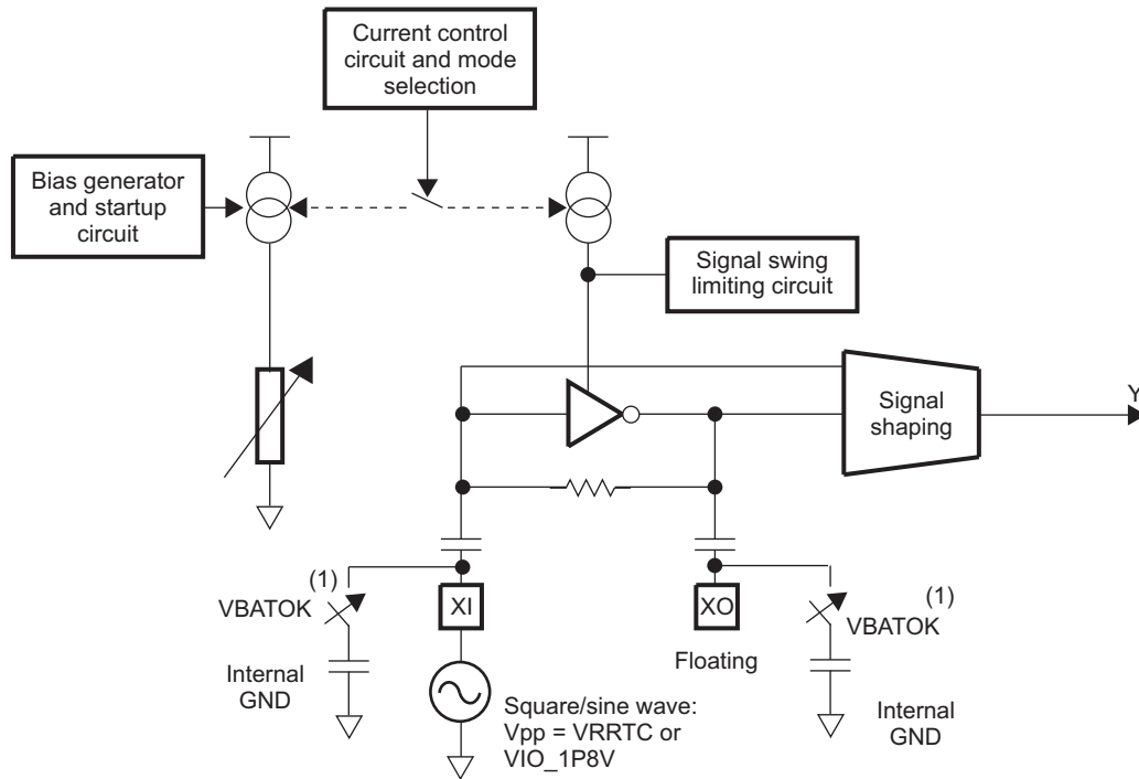
Figure 5-68. 32-kHz Oscillator Block Diagram Without Crystal Option 2
