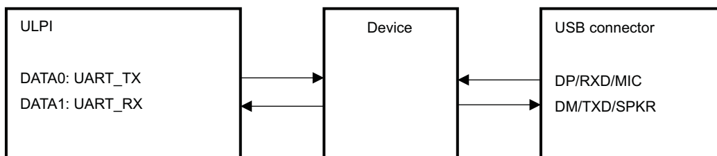
Figure 5-15. USB UART Data Flow
