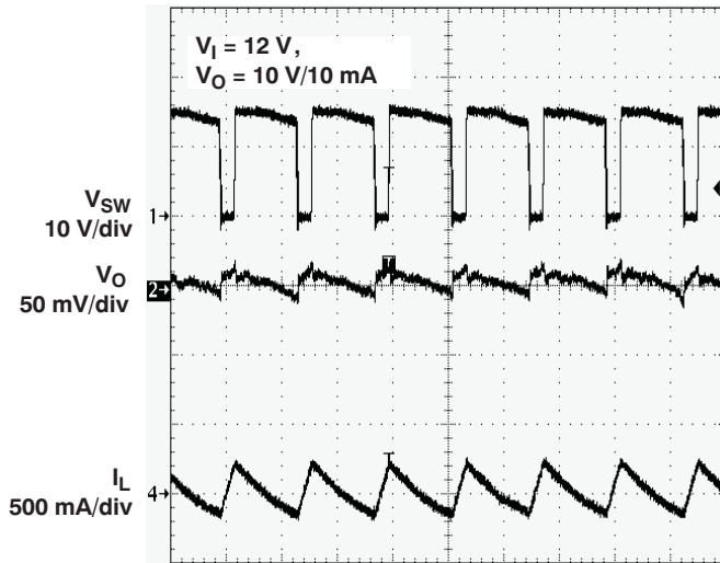
1 \mu\text{s/div} Figure 5.
