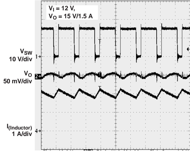
1 \mu\text{s/div} Figure 4.
