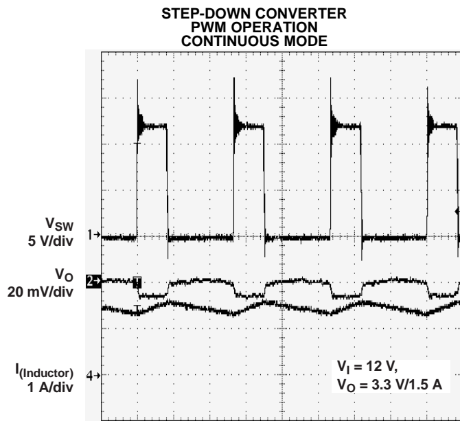
500 ns/div Figure 9.
