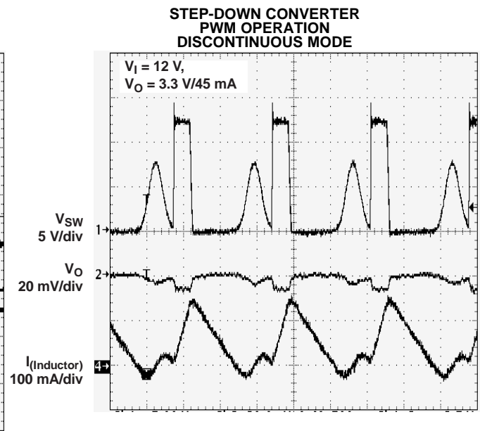
500 ns/div Figure 10.
