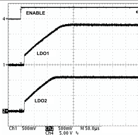
Figure 23. Start-Up LDO1 and LDO2
