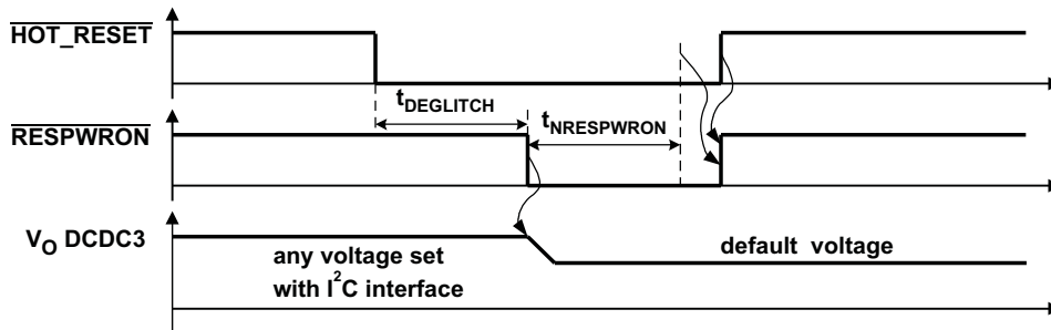
Figure 1. HOT_RESET Timing
