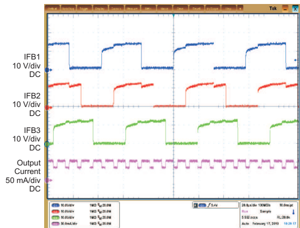
Figure 5. Switch Waveform
