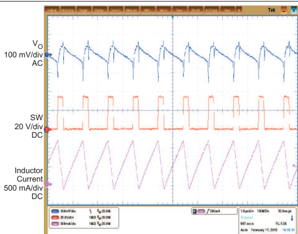
Figure 3. Switching Frequency
