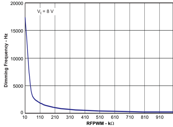
Figure 4. Dimming Frequency
