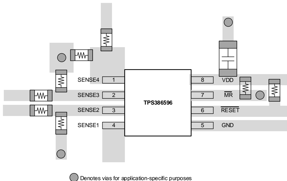
Figure 20. Example Layout (DGK Package)
