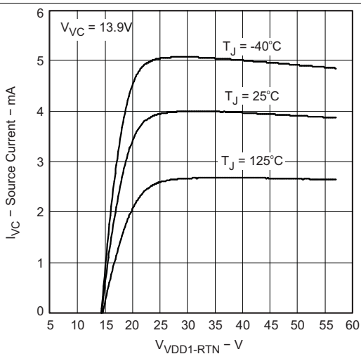
Figure 6. '754 Converter Start-Up Current vs V_{VDD1}
