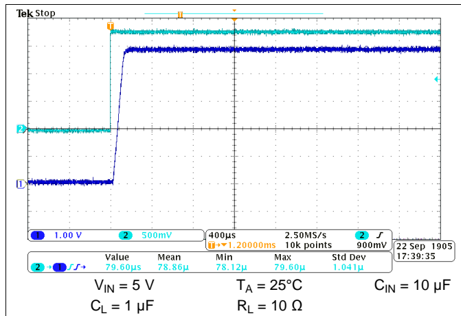
Figure 67. Turn-on Response
