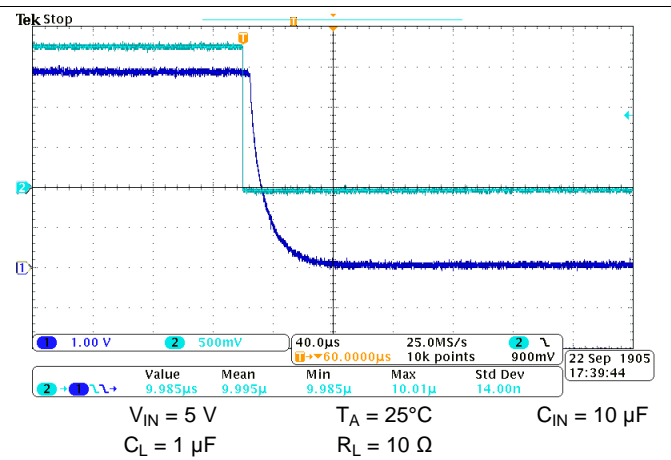
Figure 68. Turn-off Response
