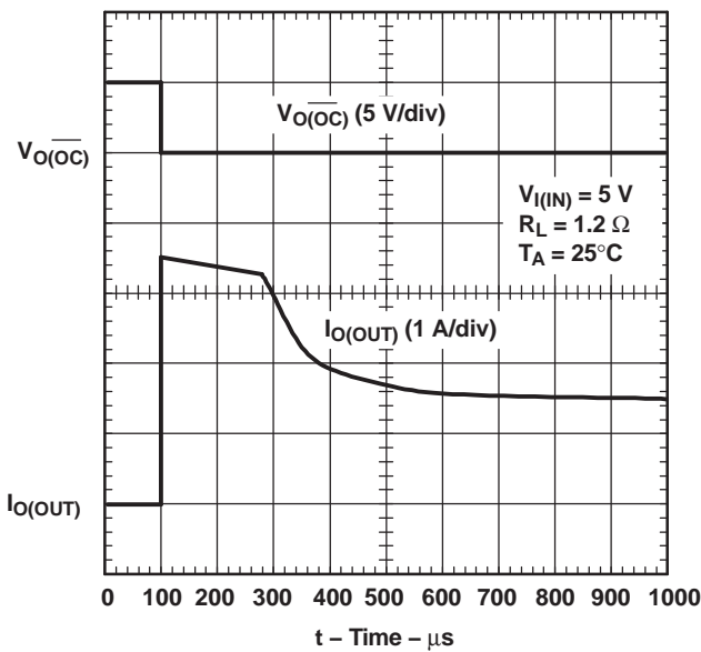
Figure 18. 1.2- \Omega Load Connected to an Enabled TPS2022 Device
