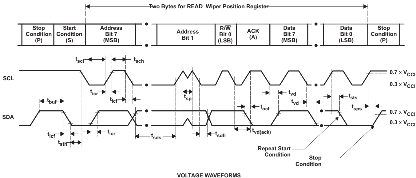
VOLTAGE WAVEFORMS
