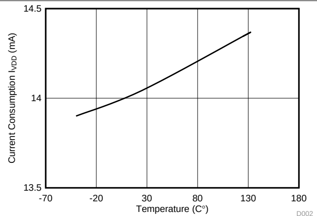
Figure 4-3. Current Consumption from VDD vs Temperature
