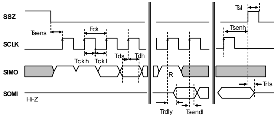
Figure 3. Serial Port Read Timings (Advanced Read Mode)
