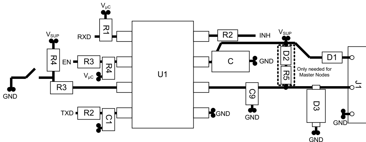
Figure 13. TPIC1021A-Q1 Layout
