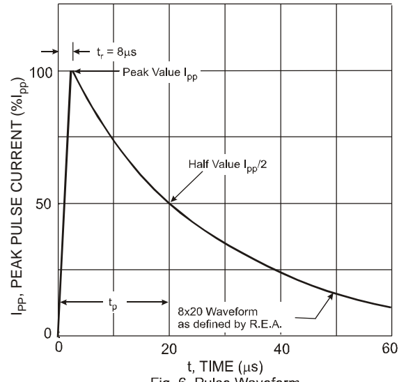
Fig. 6 Pulse Waveform
