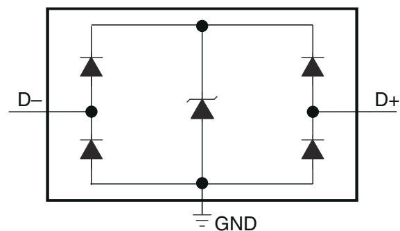
TPD2EUSB30/A Circuit
