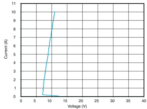
Figure 6-4. D+,D- Transmission Line Pulsers Plot for TPD2EUSB30 (100 ns Pulse, 10 ns Rise Time)
