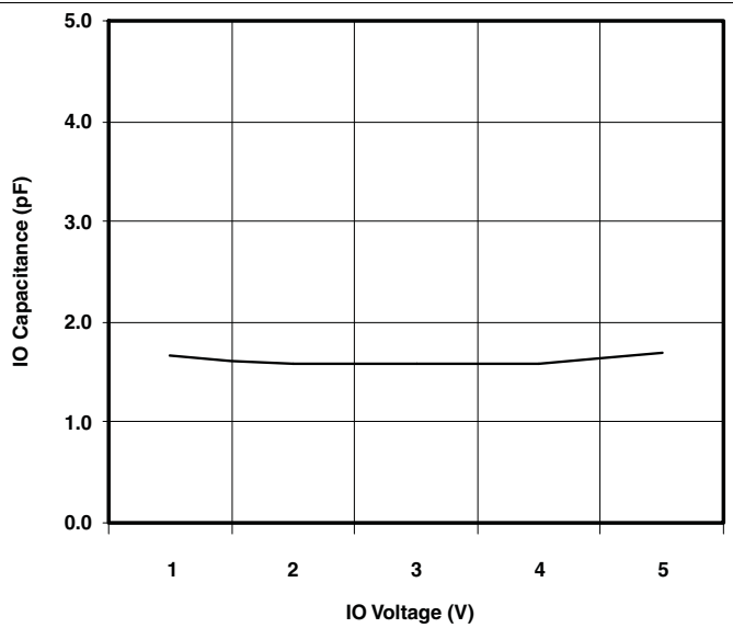
Figure 4. IO Capacitance vs Input Voltage ( V_{CC} = 5\text{ V} )
