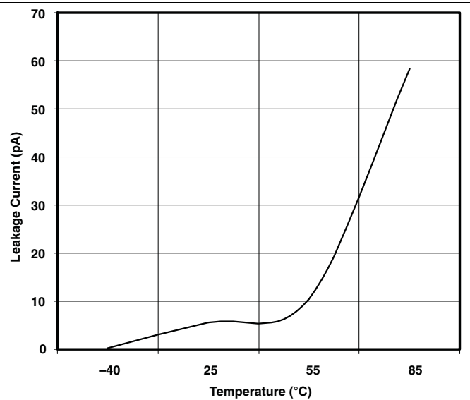
Figure 2. Leakage Current vs Temperature ( V_{IO} = 2.5\text{ V} )
