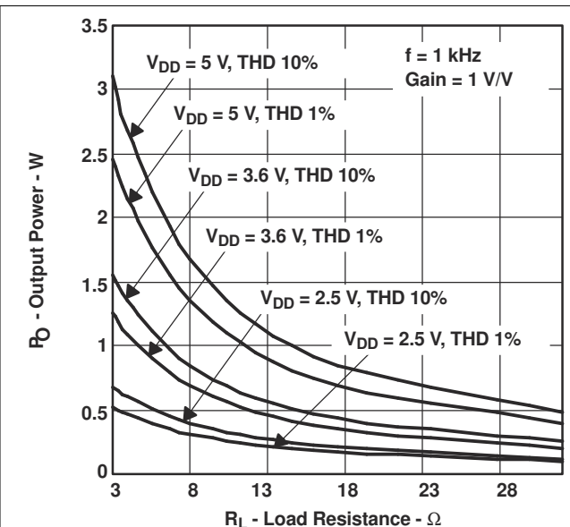
Figure 5-2. Output Power vs Load Resistance
