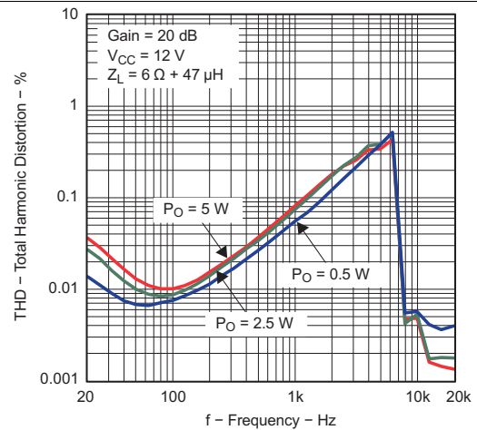
Figure 4. Total Harmonic Distortion vs Frequency (BTL)
