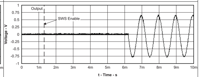
Figure 30. Start-Up Time
