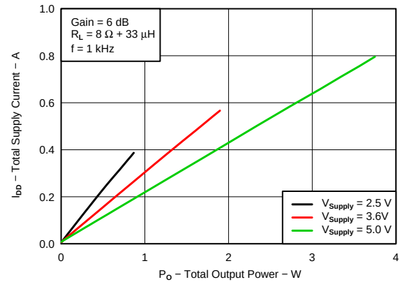
Figure 24. Total Supply Current vs Total Output Power, 8 \Omega
