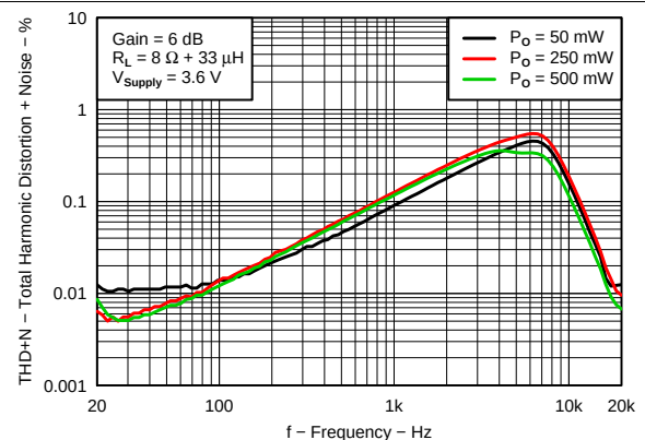
Figure 14. Total Harmonic Distortion + Noise vs Frequency V_{\text{SUPPLY}} = 3.6\ \text{V}, 8\ \Omega
