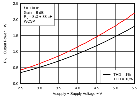
Figure 26. Output Power vs Supply Voltage, 8 \Omega
