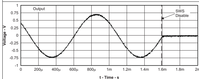
Figure 29. Shutdown Time
