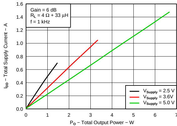
Figure 23. Total Supply Current vs Total Output Power, 4 \Omega
