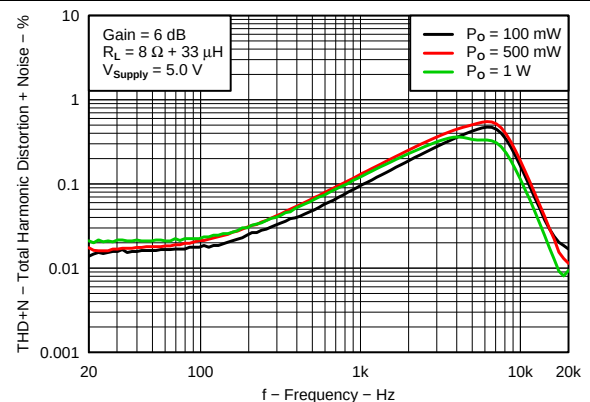
Figure 16. Total Harmonic Distortion + Noise vs Frequency V_{\text{SUPPLY}} = 5\ \text{V}, 8\ \Omega
