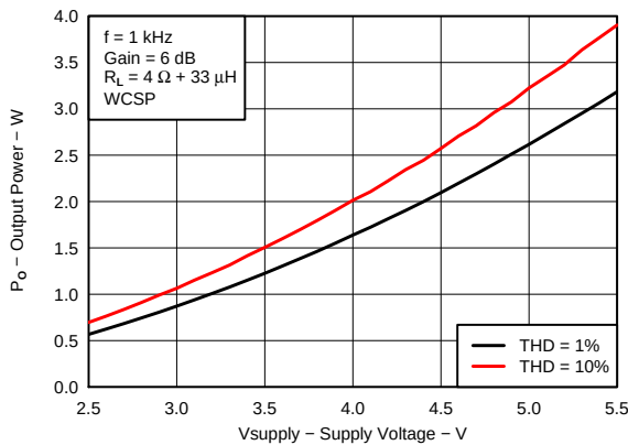
Figure 25. Output Power vs Supply Voltage, 4 \Omega
