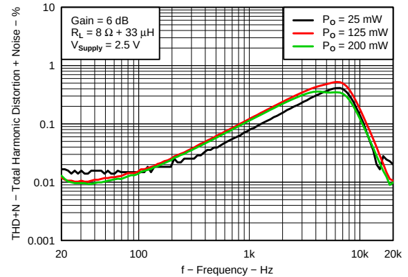
Figure 12. Total Harmonic Distortion + Noise vs Frequency V_{\text{SUPPLY}} = 2.5\ \text{V}, 8\ \Omega
