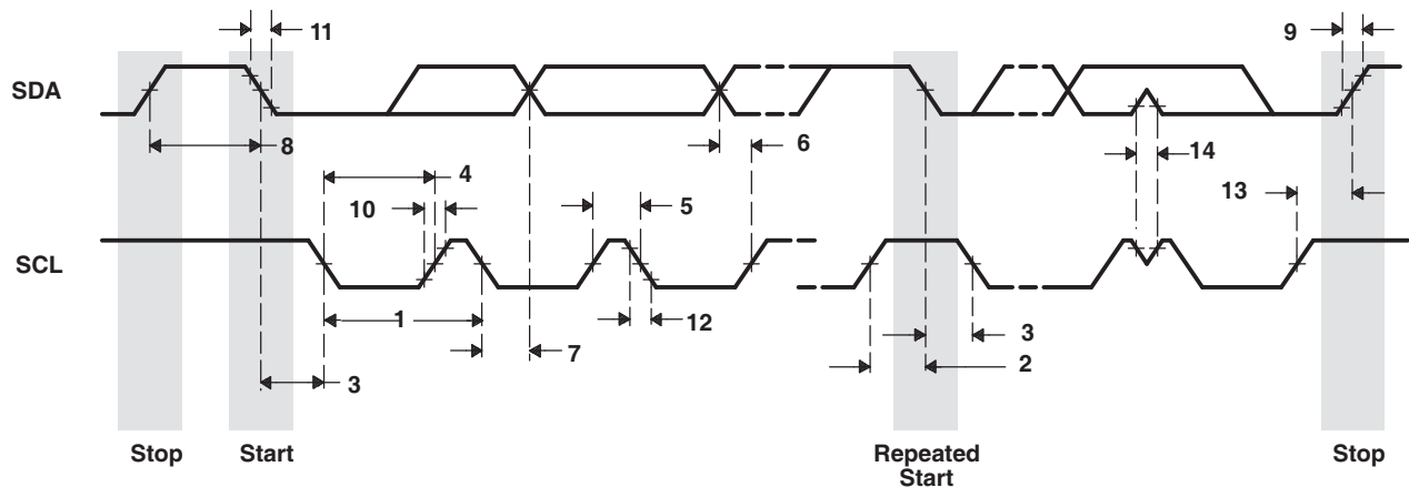
Figure 7-89. I2C Receive Timings
