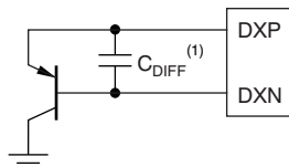
Figure 20. DIFFERENTIAL CAPACITANCE CONFIGURATION
