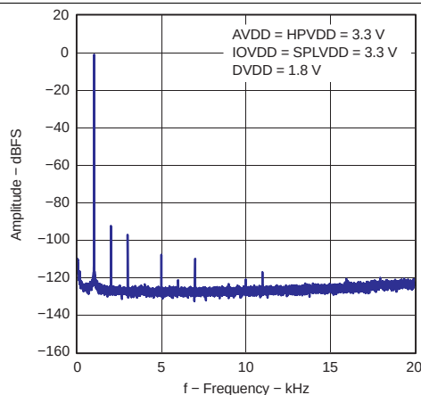
Figure 5-7. FFT – ADC Single-Ended Input
