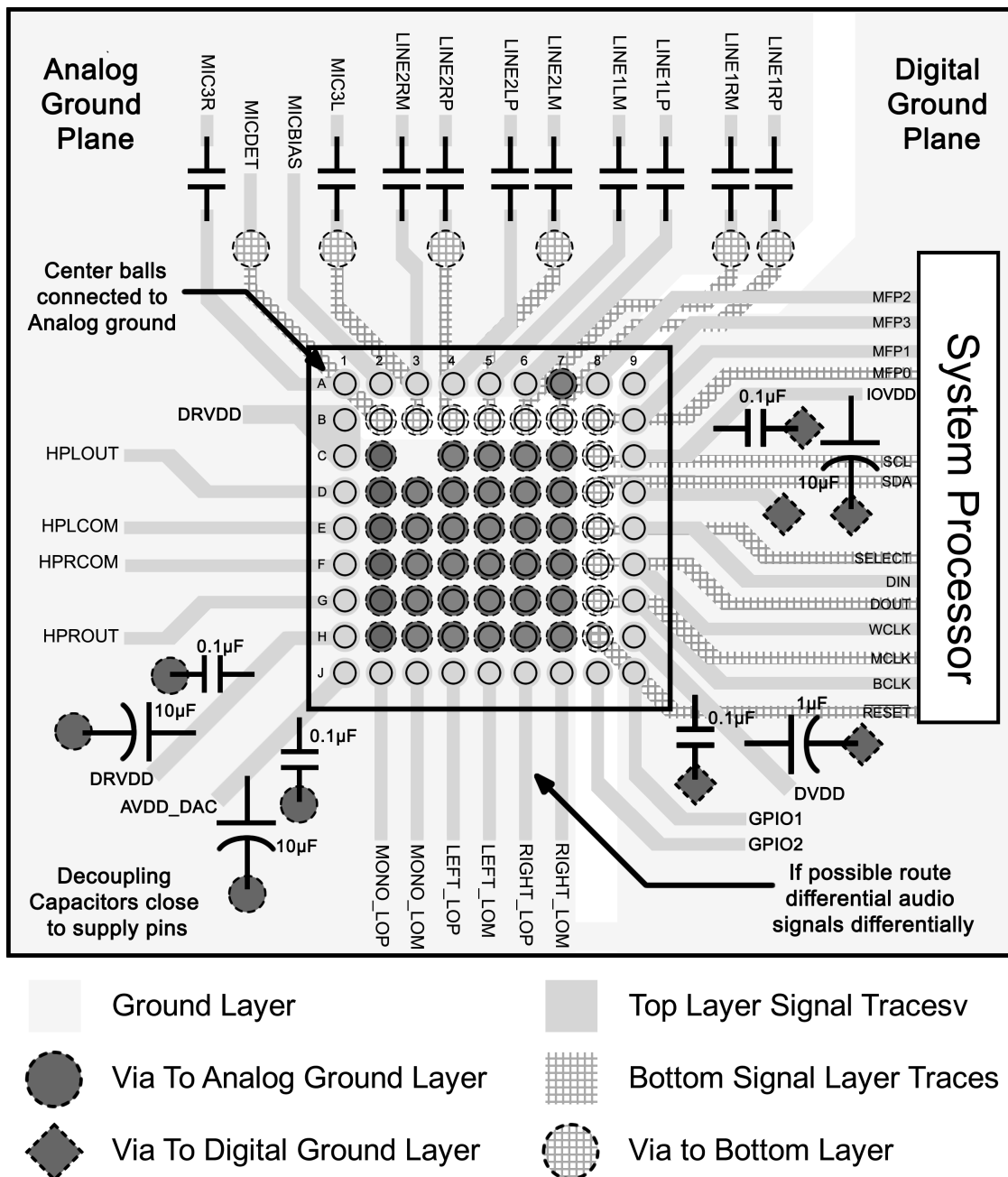
Figure 44. AIC3106 BGA Layout Example
