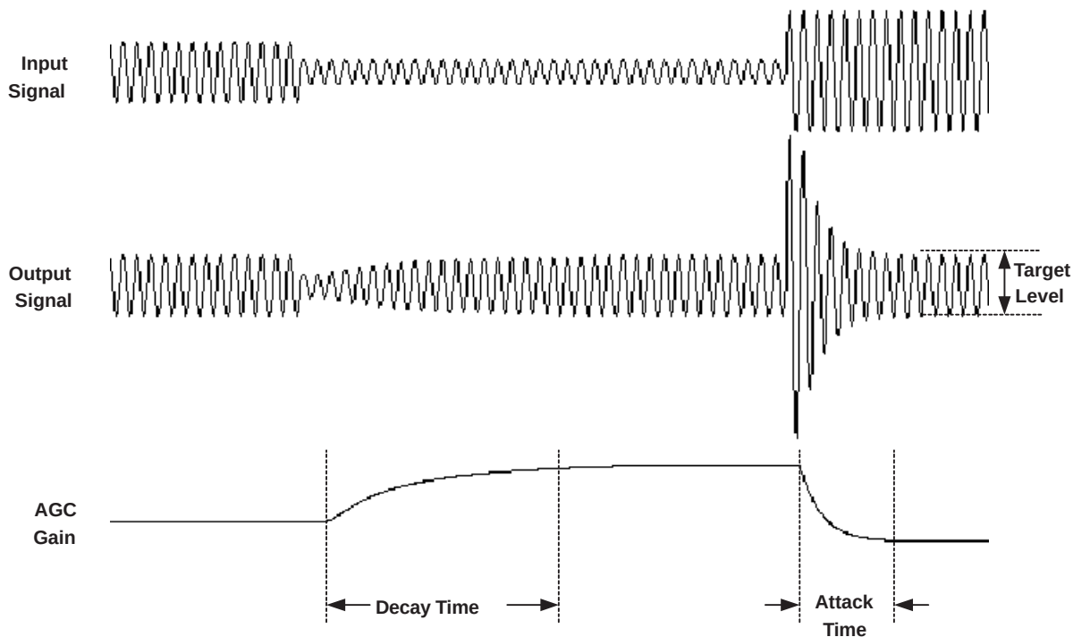
Figure 21. Typical Operation of the AGC Algorithm During Speech Recording
